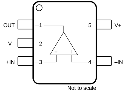
DBV Package: OPA196 5-Pin SOT Top View
