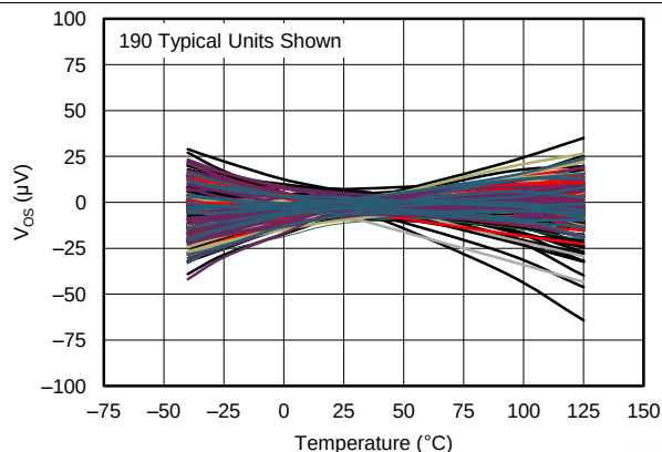
Figure 7. Offset Voltage Drift Distribution
