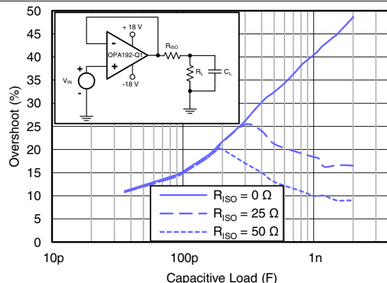
Figure 56. Small-Signal Overshoot vs Capacitive Load (100-mV Output Step)
