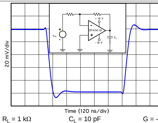
Figure 34. Negative Overload Recovery
