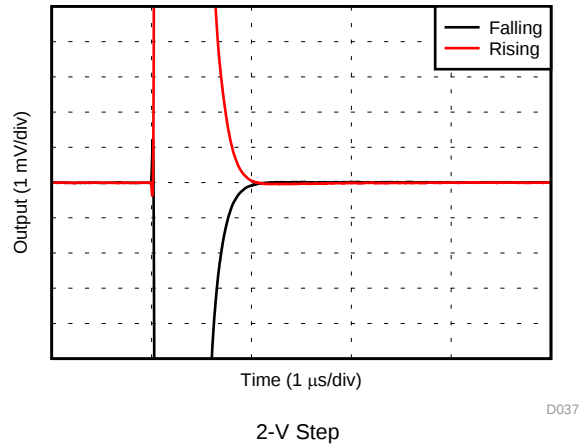
Figure 27. Settling Time
