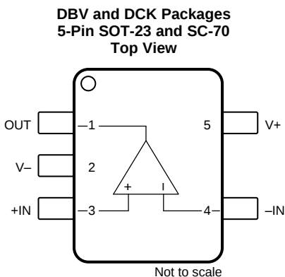
Pin Functions
