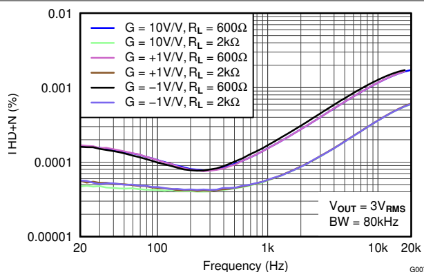
Figure 5-7. THD+N Ratio vs Frequency
