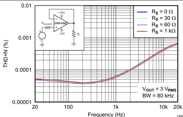
Figure 5-9. THD+N Ratio vs Frequency
