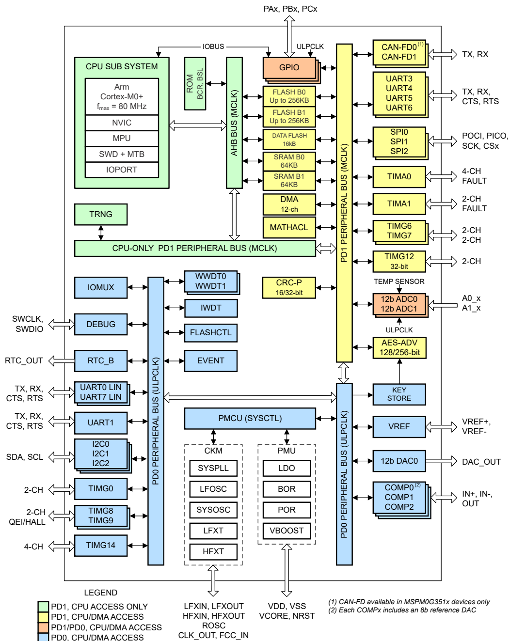
Figure 4-1. MSPM0G352x-Q1 Functional Block Diagram
