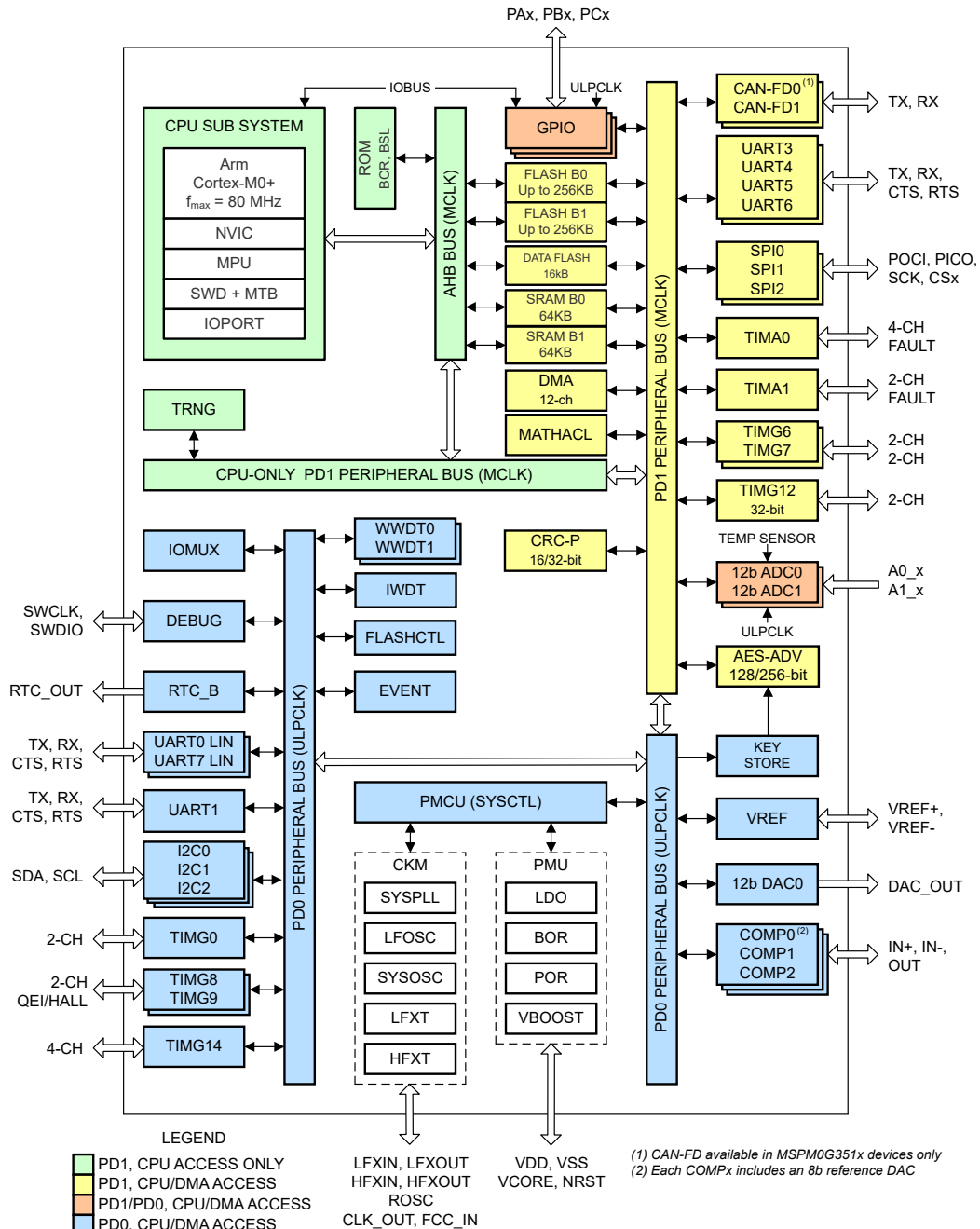
Figure 8-1. MSPM0G352x-Q1 Functional Block Diagram
