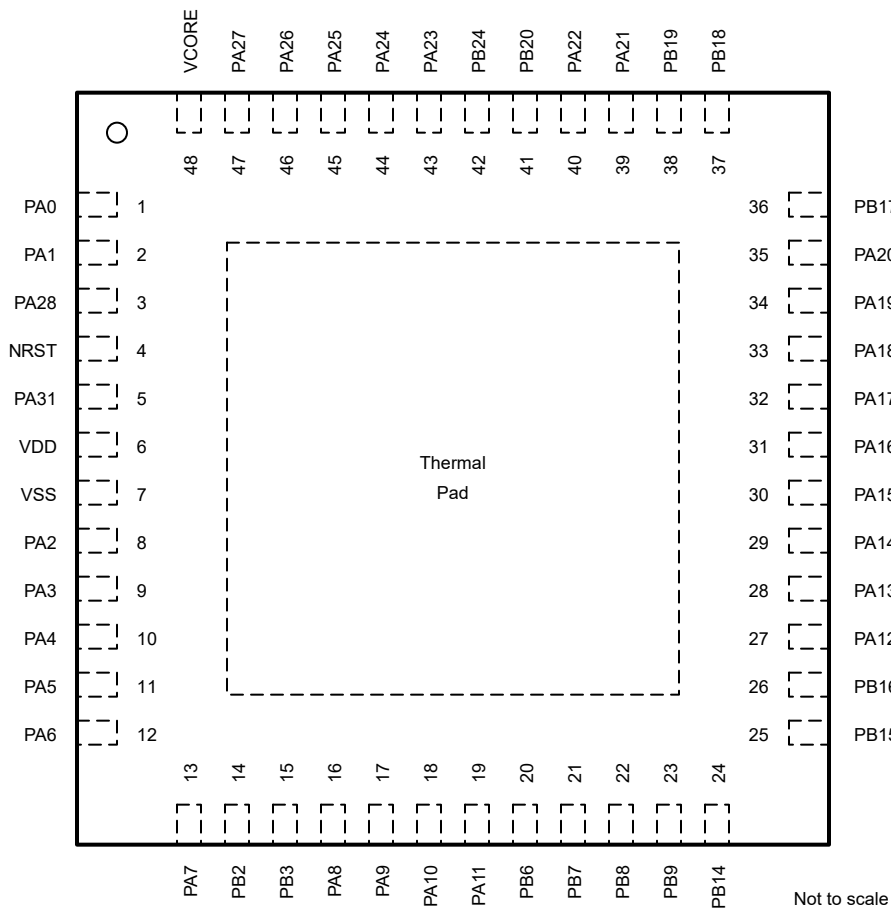
Figure 6-5. 48-pin RGZ (0.5mm) (VQFN) Package Diagram
