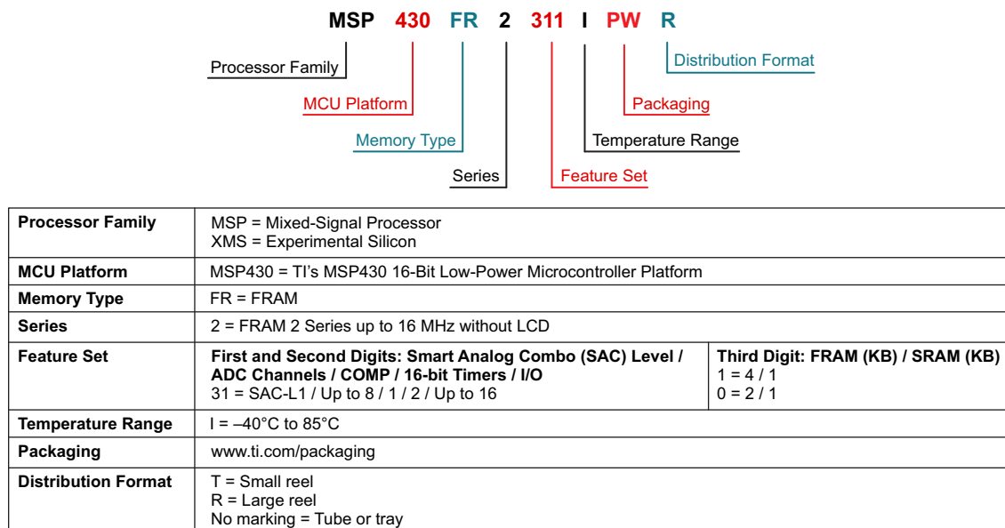
Figure 8-1. Device Nomenclature
