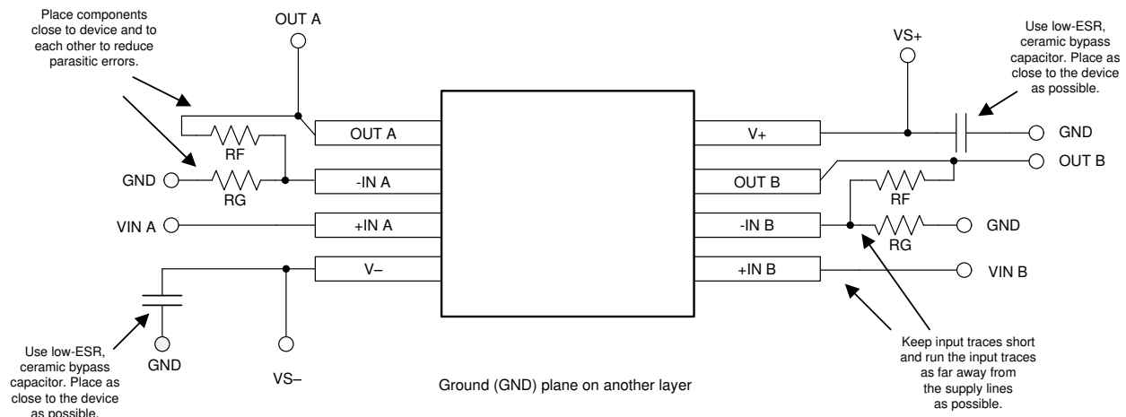
Figure 37. Layout Example
