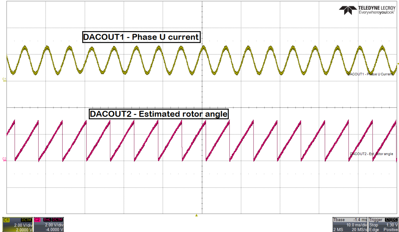
Figure 10-10. DACOUT1 and DACOUT2
