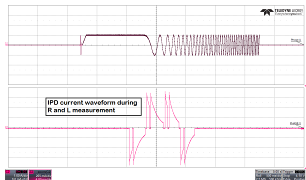
Figure 10-4. IPD current waveform during R and L measurement
