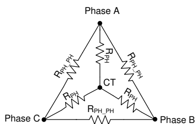
Figure 7-46. Motor Resistance
