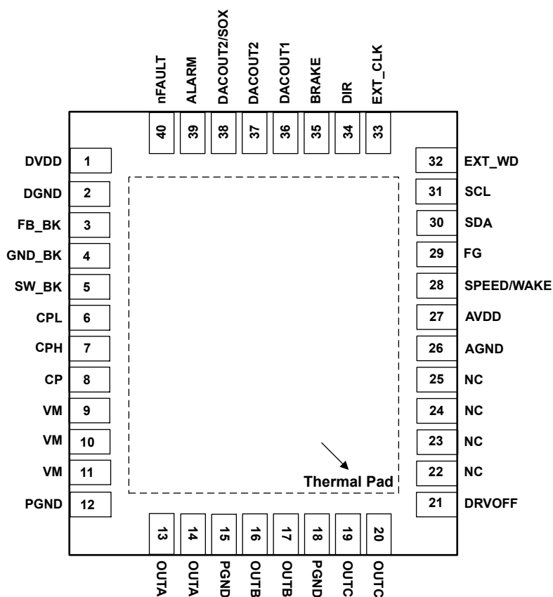
Figure 4-1. MCF8315C-Q1, 40-Pin RGF VQFN With Exposed Thermal Pad, Top View
