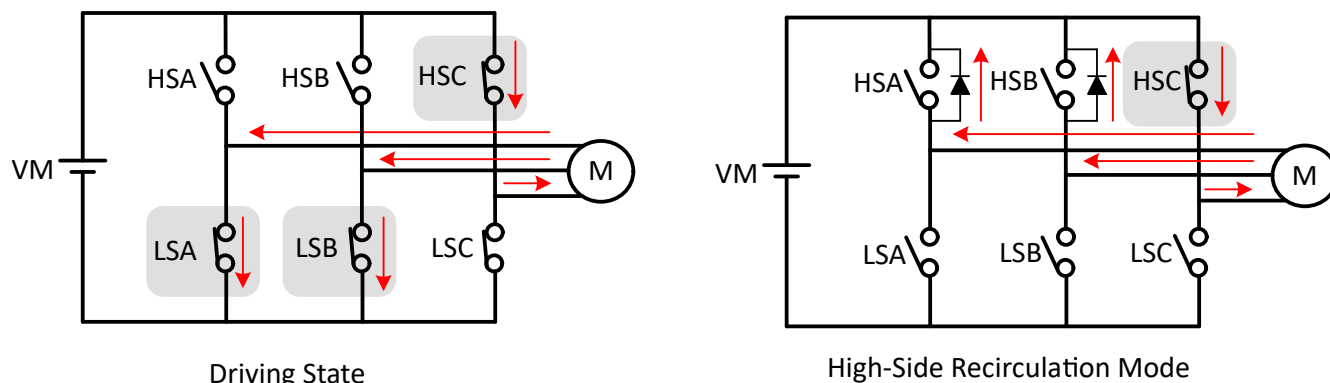
Figure 7-46. High-Side Recirculation
