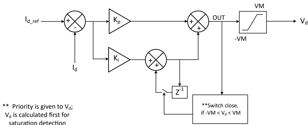
Figure 7-36. I_d Current PI Control
