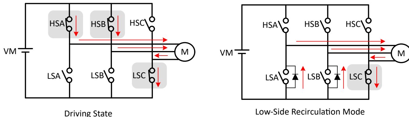
Figure 7-45. Low-Side Recirculation
