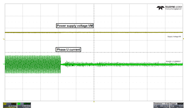
Figure 8-11. Power supply voltage and phase current waveform when AVS is enabled
