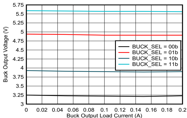
Figure 6-3. Buck regulator output voltage over load current
