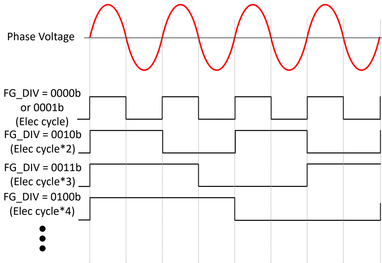
Figure 7-49. FG Frequency Divider
