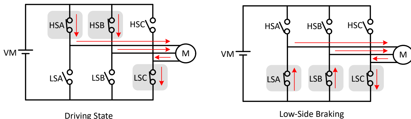
Figure 7-47. Low-Side Braking
