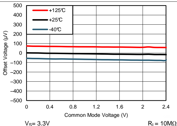
Figure 12. Typical Offset Voltage vs. Common Mode Voltage
