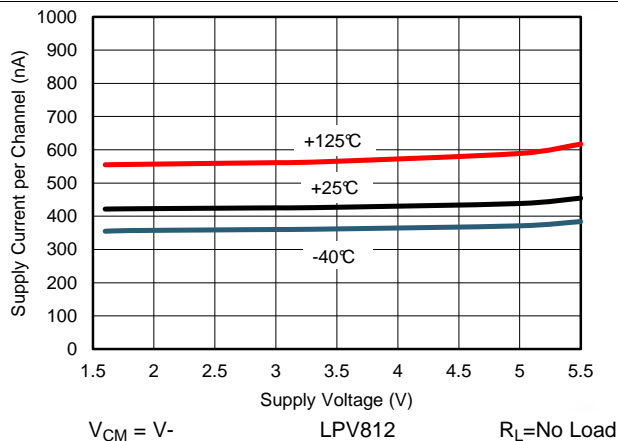
Figure 10. Supply Current vs. Supply Voltage, LPV812
