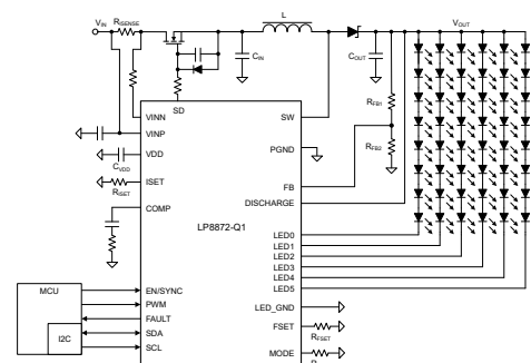
Simplified Schematic
