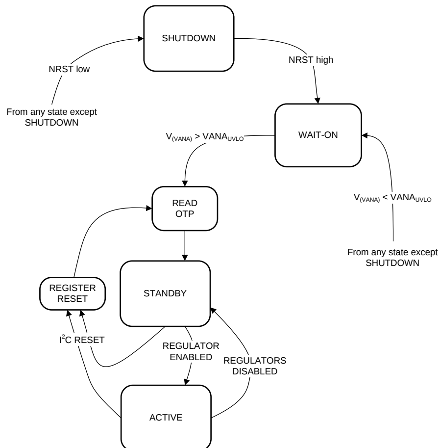
Figure 12. Device Operation Modes
