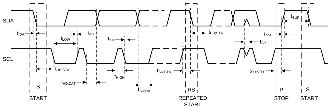
Figure 15. I²C-Compatible Timing
