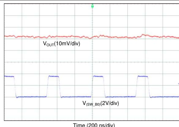
Figure 81. Output Voltage Ripple, Forced-PWM Mode (4-Phase Output)
