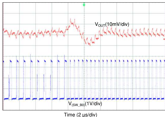
Figure 88. Transient from PFM-to-PWM Mode (1-Phase Output)
