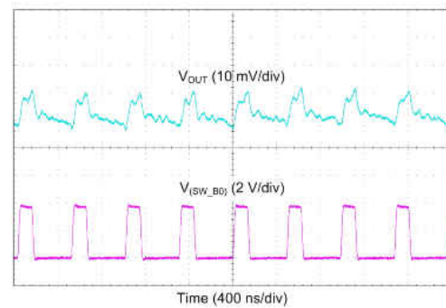
Figure 8-13. Buck Output Voltage Ripple, Forced PWM Mode
