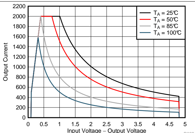
Figure 18. Recommended Continuous Operating Area for V_{OUT} = 1.2 V
