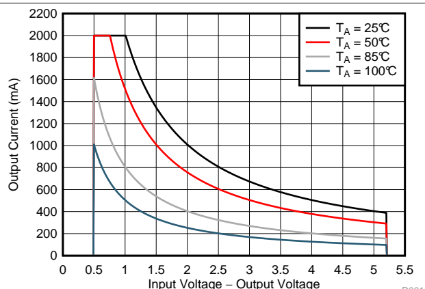
Figure 17. Recommended Continuous Operating Area for V_{OUT} = 0.8 V
