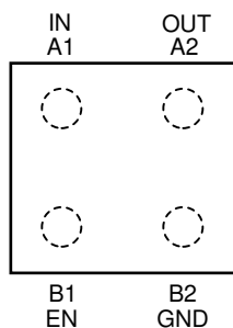
Figure 5-1. YKA Package, 4-Pin Ultra-Thin DSBGA, Top View
