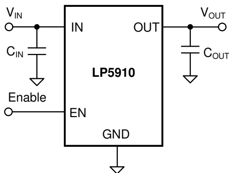
Simplified Schematic
