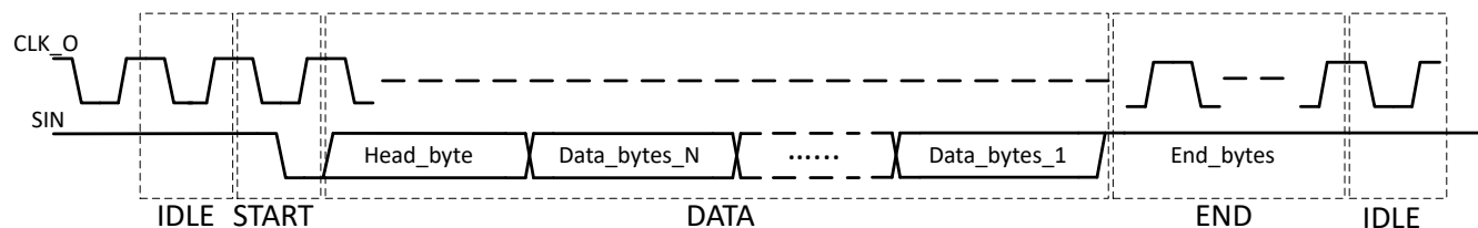
Figure 7-2. Command Format
