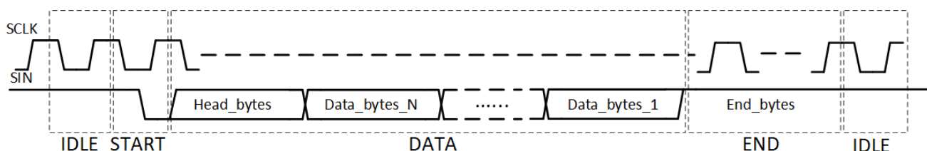
Figure 6-14. CCSI Frame
