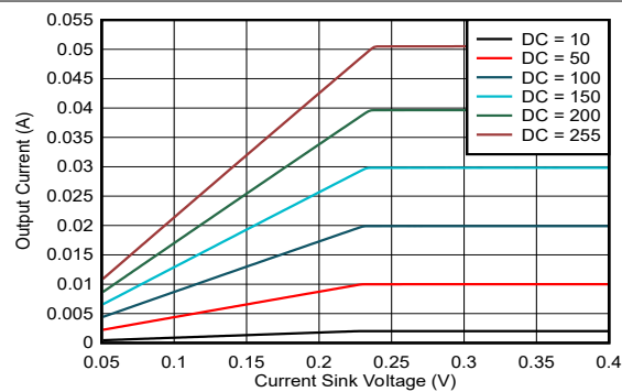
Figure 6-5. Current Sinks Voltage vs Current (MC = 1, VCC = 3.6V)
