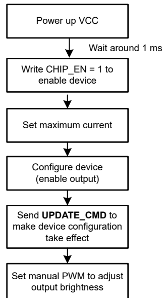
Figure 8-2. Program Procedure
