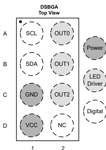
Figure 5-2. LP5817 YCH Package 8-Pin DSBGA Top View
