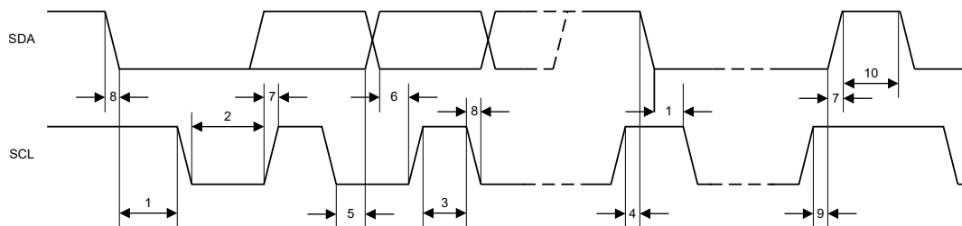
Figure 6-1. I²C Timing Parameters
