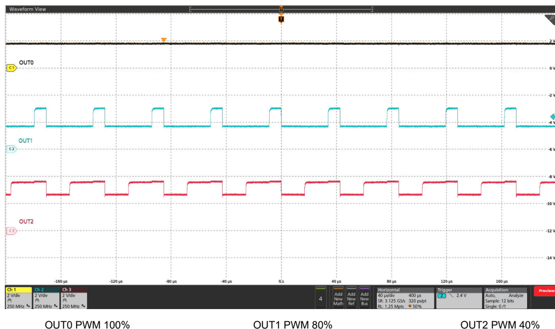
Figure 8-3. Current Sinks Waveforms of OUT0, OUT1, OUT2
