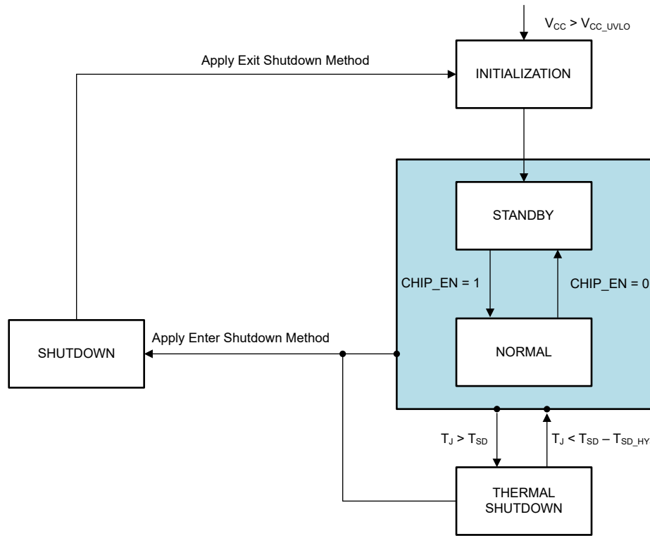
Figure 7-4. Functional Modes
