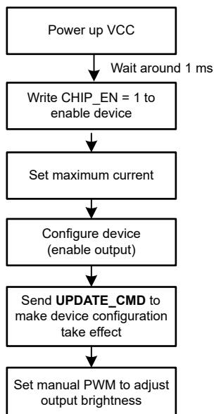
Figure 8-2. Program Procedure
