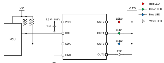
LP5816 Simplified Schematic
