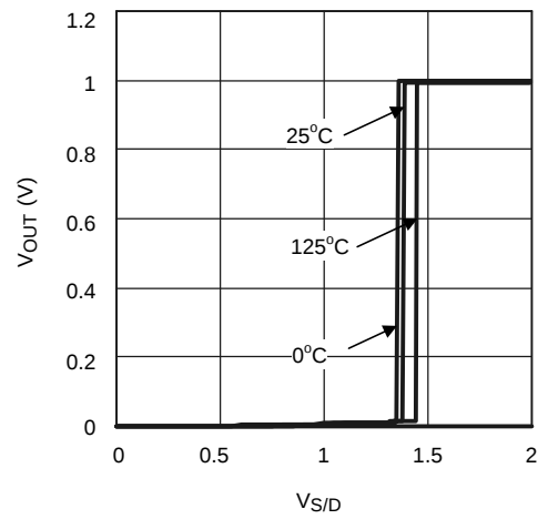
Figure 26. Turnoff Characteristics
