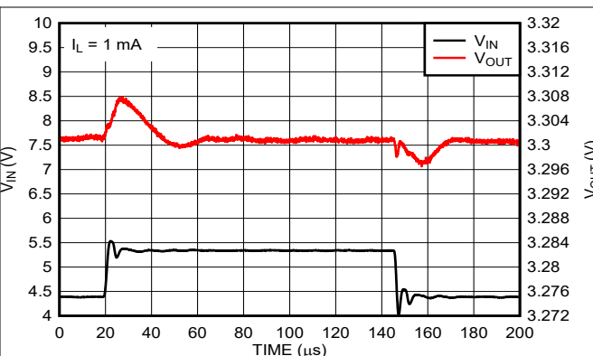
Figure 7-8. Line Transient Response (New Chip)
