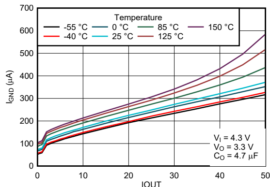
Figure 6-18. Ground Pin Current vs Load Current for New Chip
