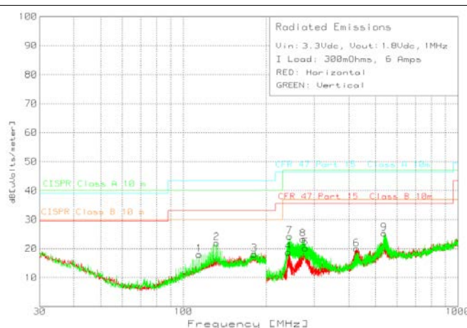
Figure 35. Radiated Emissions 3.3-V Input, 1.8-V Output, 6-A Load (EN55022 Class B)
