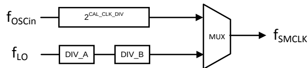
Figure 49. Block Diagram of SM Clock
