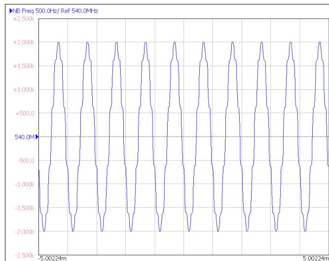
Figure 84. Simulated FM Modulation (10 times over-sampling)
