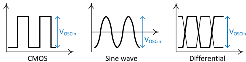
Figure 55. Input Clock Definition
