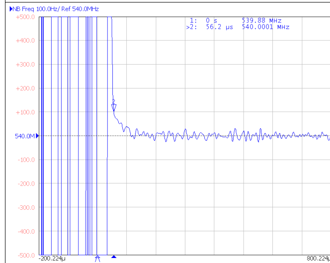
Figure 82. External VCO to Internal VCO Switching Time
