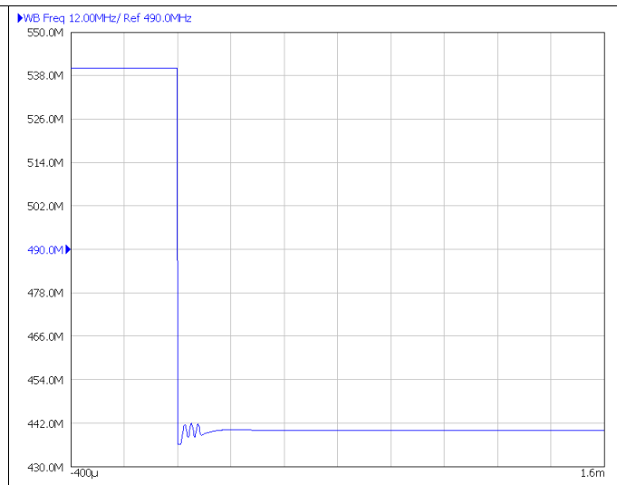
Figure 81. Internal VCO to External VCO Switching
