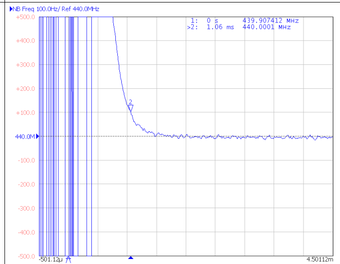
Figure 83. Internal VCO to External VCO Switching Time
