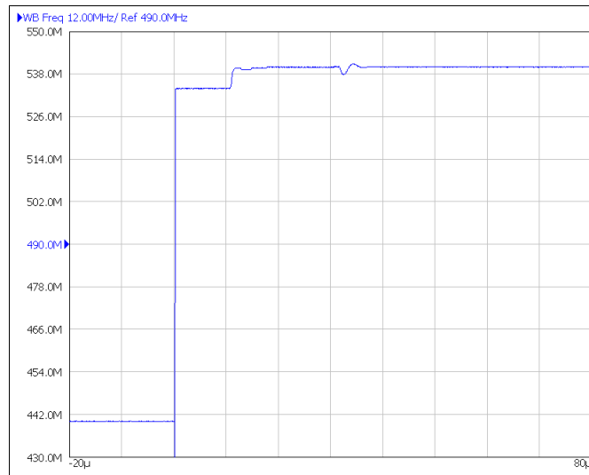
Figure 80. External VCO to Internal VCO Switching
