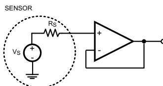
High Impedance Sensor Interface CMOS Input Feature
