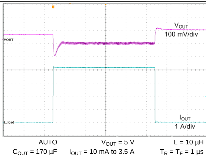
Figure 33. Load Transients
