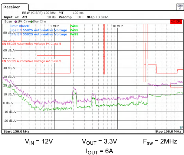
Figure 8-35. Conducted EMI vs CISPR 25 Limits (Pink: Peak Signal, Green: Average Signal)
