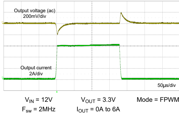
Figure 8-26. Load Transient
