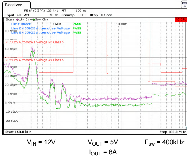
Figure 8-36. Conducted EMI vs CISPR 25 Limits (Pink: Peak Signal, Green: Average Signal)
