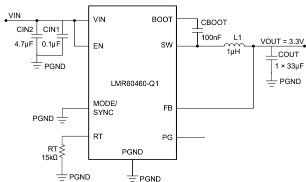
Figure 8-46. Fixed Output Version Schematic - 2.2MHz 3.3V
