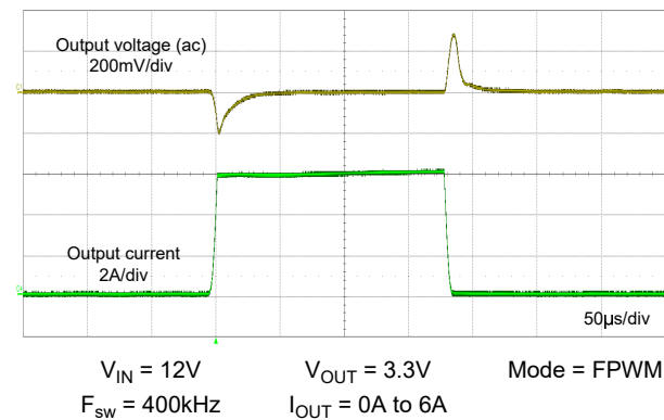
Figure 8-24. Load Transient
