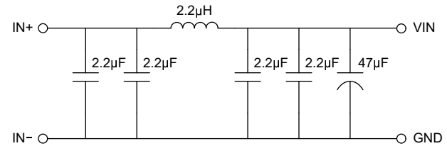
Figure 8-43. Recommended input EMI filter
