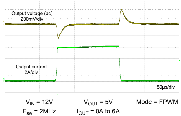
Figure 8-27. Load Transient
