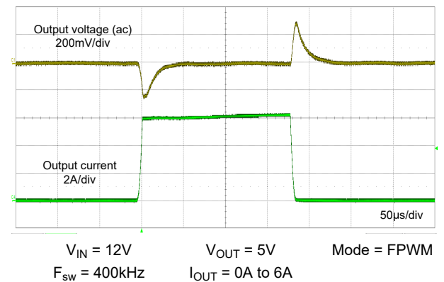
Figure 8-25. Load Transient
