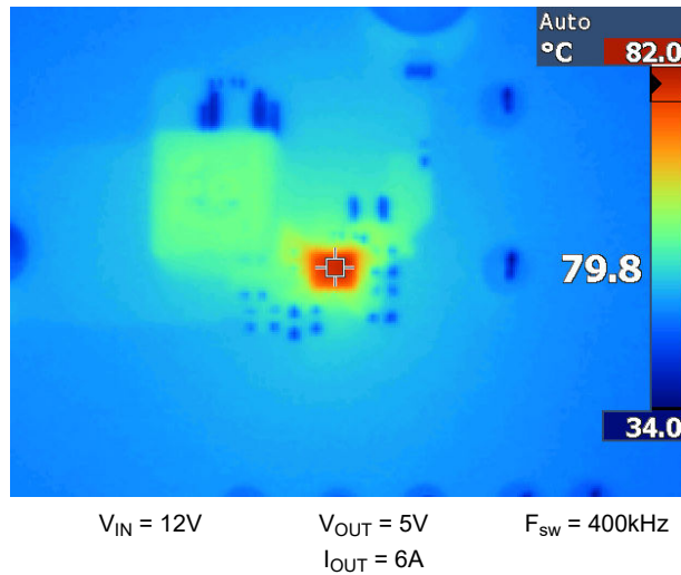
Figure 8-42. EVM Thermal Performance
