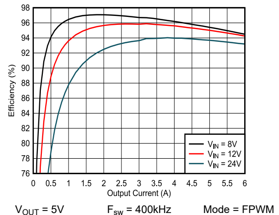
Figure 8-5. Efficiency - FPWM Mode
