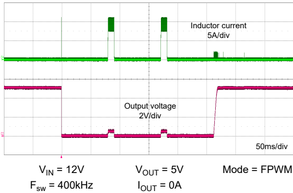
Figure 8-32. Short-Circuit Behavior
