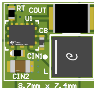
Figure 8-47. Ultra-Compact Fixed Output Voltage Configuration EVM Layout
