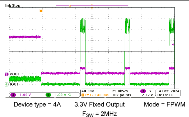
Figure 8-9. Short-Circuit Applied
