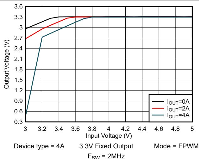
Figure 8-4. Dropout Voltage
