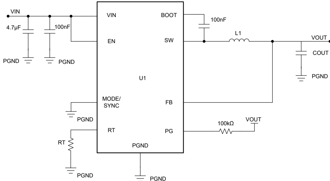
Figure 8-25. Example Application Circuit
