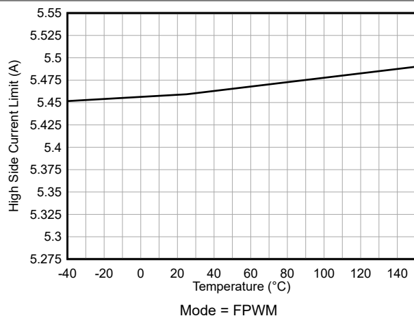
Figure 6-1. High Side MOSFET Current Limit
