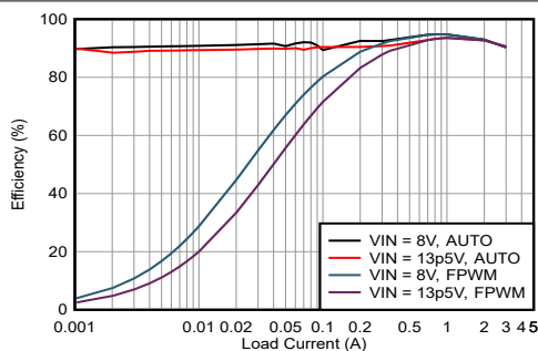
Device type = 3A 3.3V fixed output Mode = Auto/FPWM F_{SW} = 400kHz
