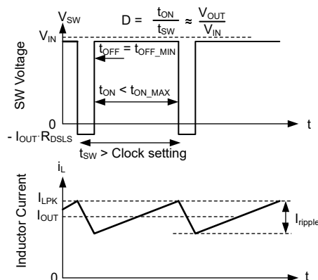
Figure 7-10. Dropout Waveforms
