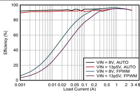
Device type = 3A 5V fixed output Mode = Auto/FPWM F_{SW} = 400kHz
