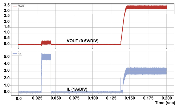
Figure 8-14. Short-Circuit Recovery
