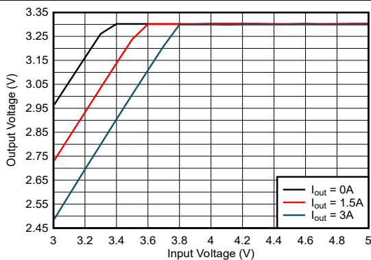
Device type = 3A 3.3V fixed output Mode = FPWM F_{SW} = 2MHz
