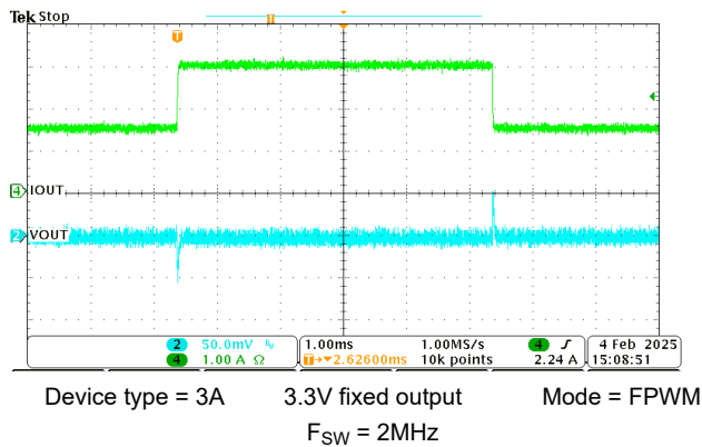
Figure 8-10. 1.5A to 3A Load Transient
