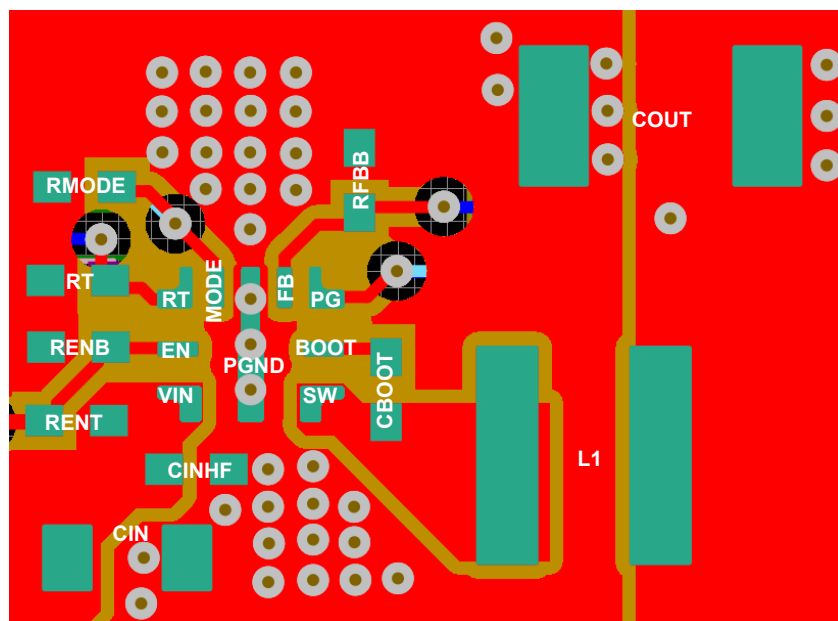
Figure 8-27. Fixed Output Version
