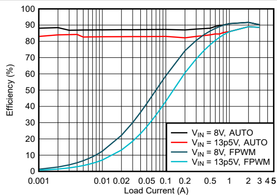
Device type = 3A 3.3V fixed output Mode = Auto/FPWM F_{SW} = 2MHz
