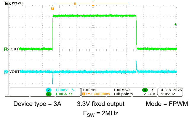
Figure 8-9. 20mA to 3A Load Transient
