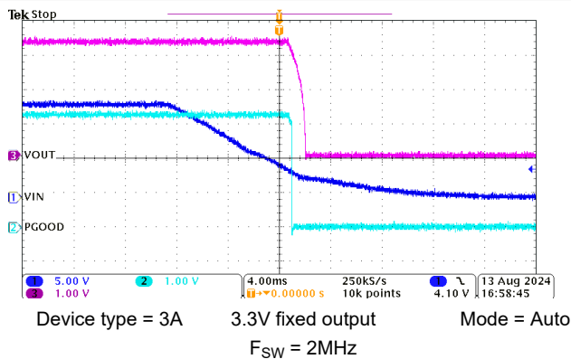
Figure 8-12. Shutdown Operation
