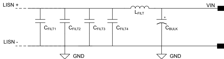
Figure 8-24. Typical Input EMI Filter Schematic
