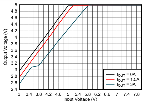
Device type = 3A 5V fixed output Mode = FPWM F_{SW} = 2MHz
