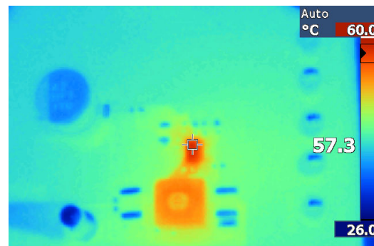
Figure 8-17. Thermal Performance
