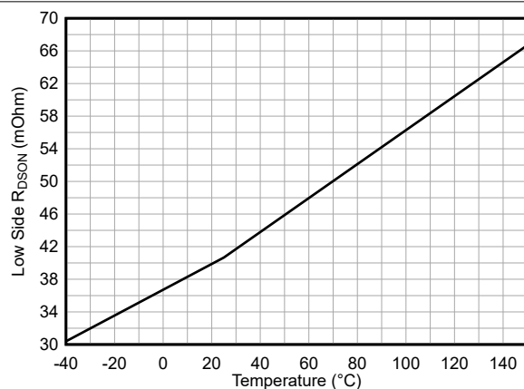
Figure 6-4. Low Side MOSFET R_{DS-ON}
