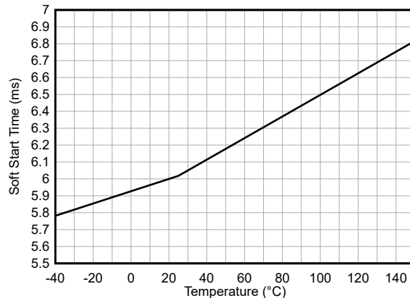
Figure 6-6. Soft-Start Time
