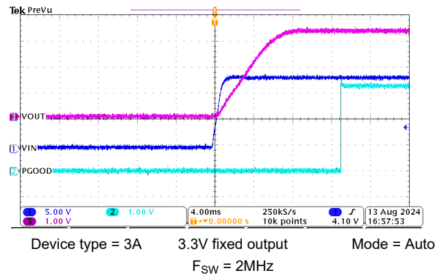
Figure 8-11. Start-Up Operation
