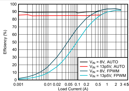
Device type = 3A 5V fixed output Mode = Auto/FPWM F_{SW} = 2MHz
