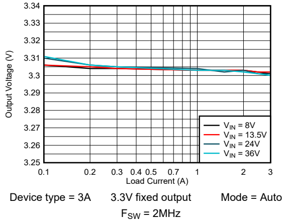
Figure 8-8. Load Regulation
