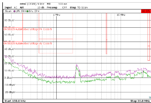
Figure 8-20. Conducted EMI versus CISPR25 Limits (Purple: Peak Signal, Green: Average Signal), LMR60440QEV
