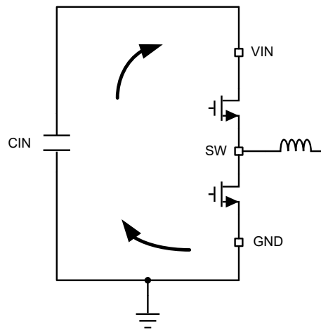
Figure 8-25. Current Loops With Fast Edges
