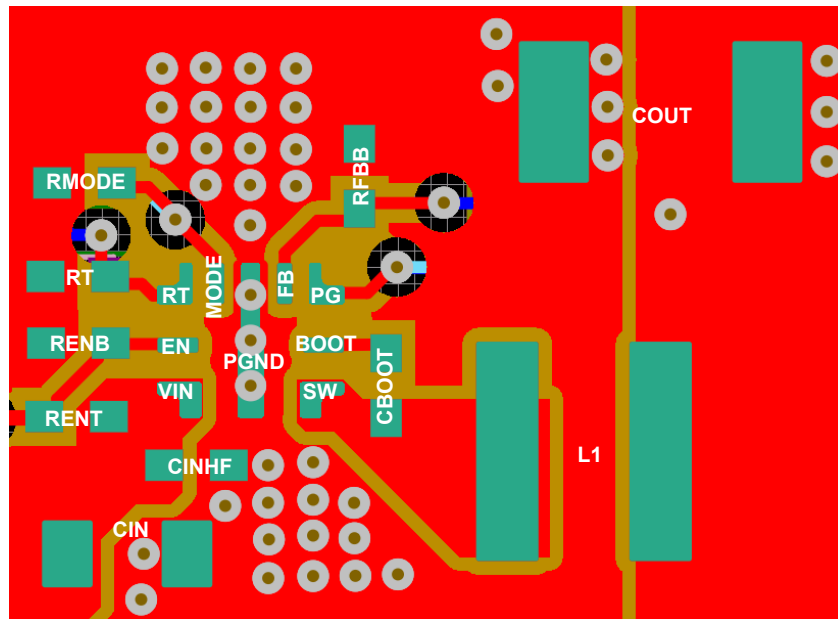
Figure 8-26. Fixed Output Version
