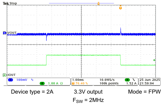
Figure 8-12. 1A to 2A Load Transient
