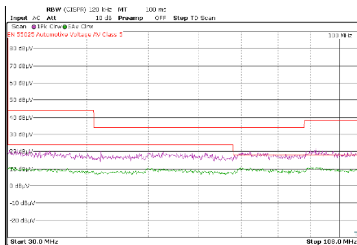
Figure 8-21. Conducted EMI versus CISPR25 Limits (Purple: Peak Signal, Green: Average Signal), LMR60440QEV
