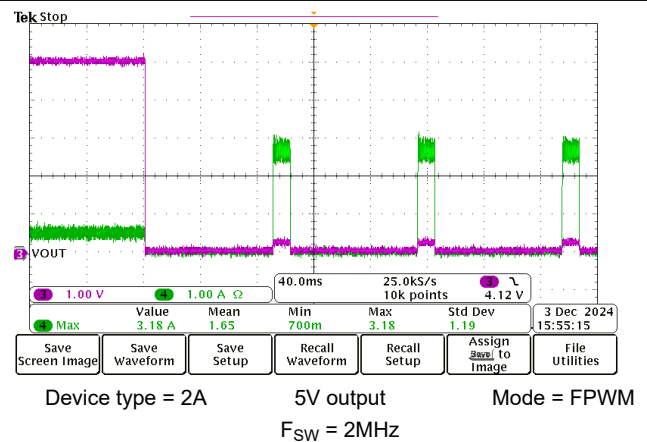
Figure 8-15. Short-Circuit Applied
