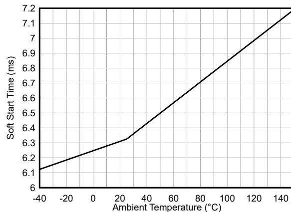
Figure 6-6. Soft-Start Time
