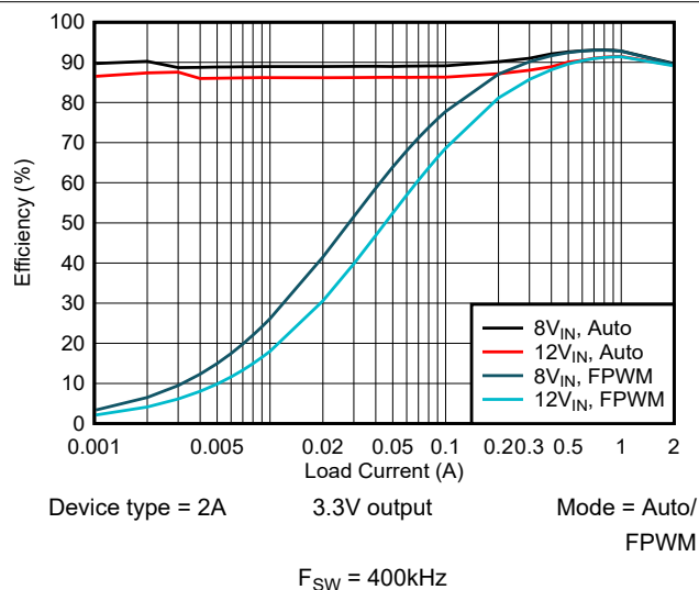
Figure 8-3. Efficiency
