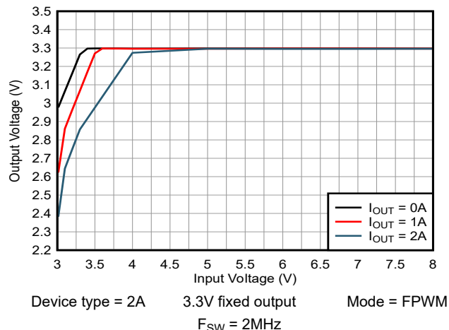
Figure 8-6. Dropout
