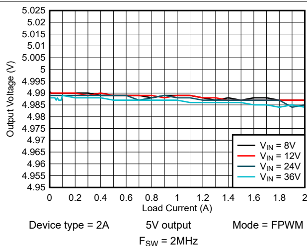
Figure 8-8. Load Regulation
