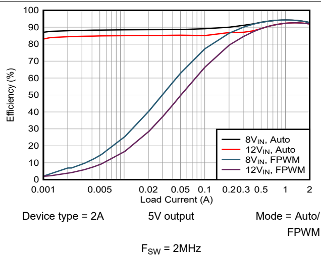
Figure 8-4. Efficiency
