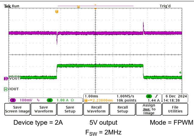
Figure 8-10. 1A to 2A Load Transient
