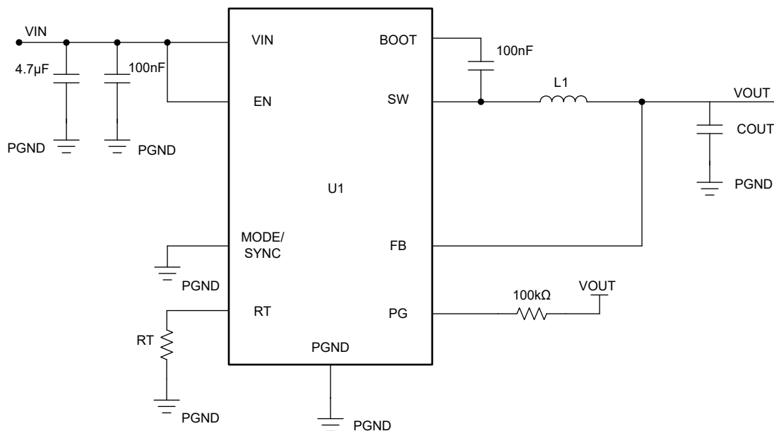
Figure 8-24. Example Application Circuit
