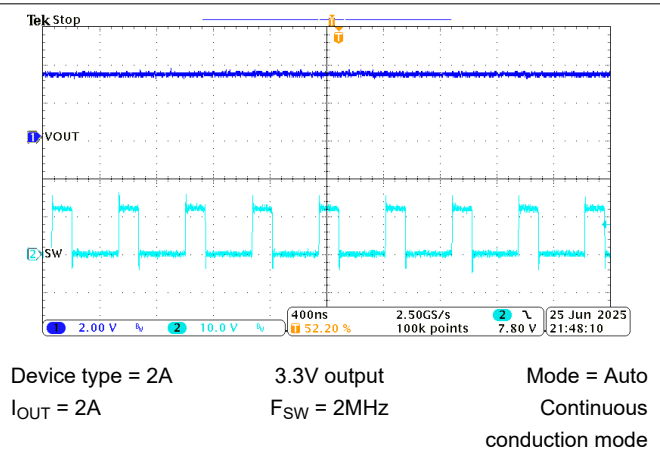
Figure 8-17. Steady State Waveform
