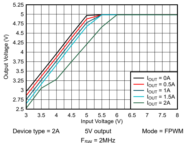
Figure 8-7. Dropout Voltage
