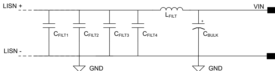
Figure 8-23. Typical Input EMI Filter Schematic
