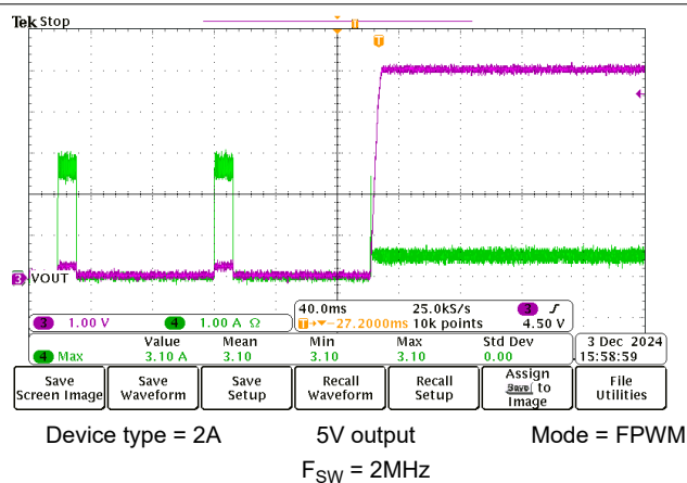
Figure 8-16. Short-Circuit Recovery
