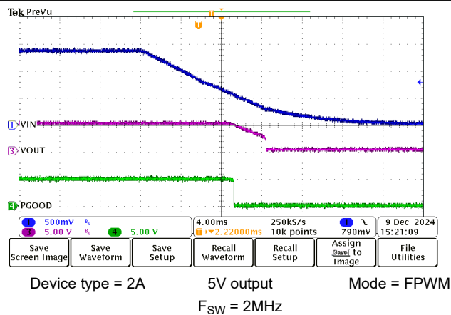
Figure 8-14. Shutdown Operation
