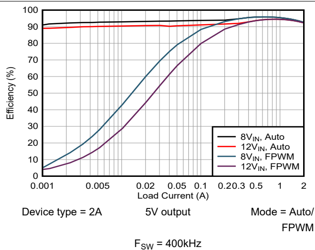
Figure 8-5. Efficiency
