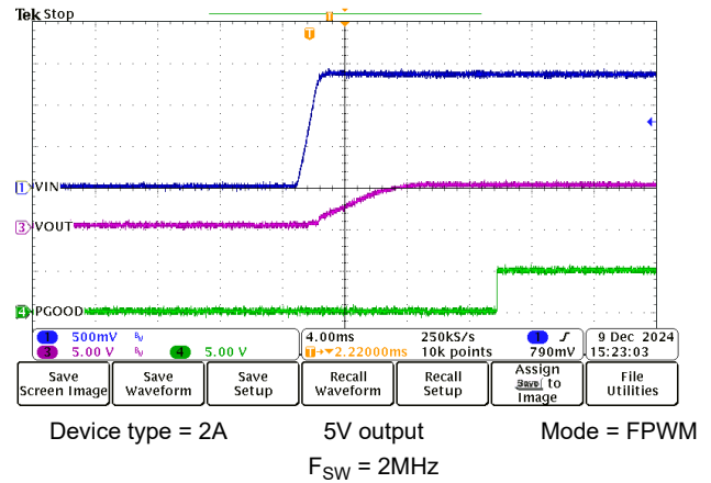
Figure 8-13. Start-Up Operation
