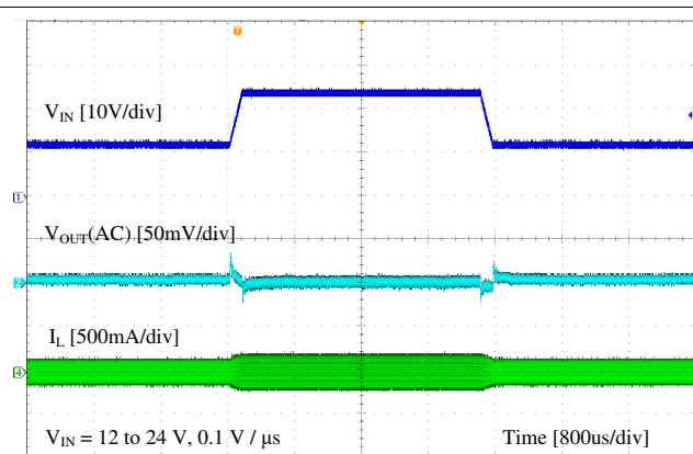
Figure 8-8. Line Transient
