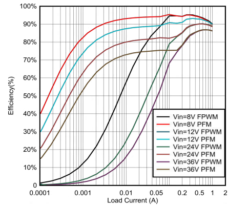
Figure 6-4. 5-V Efficiency Versus Load Current
