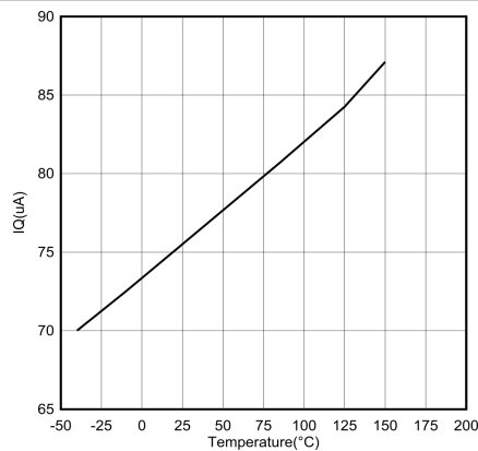
Figure 6-10. I_Q Versus Temperature
