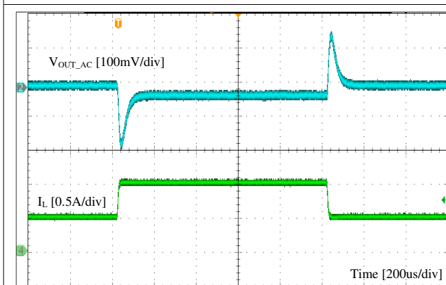
Figure 8-7. Load Transient
