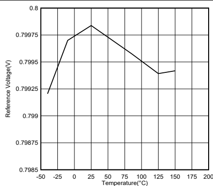
Figure 6-12. Reference Voltage Versus Temperature
