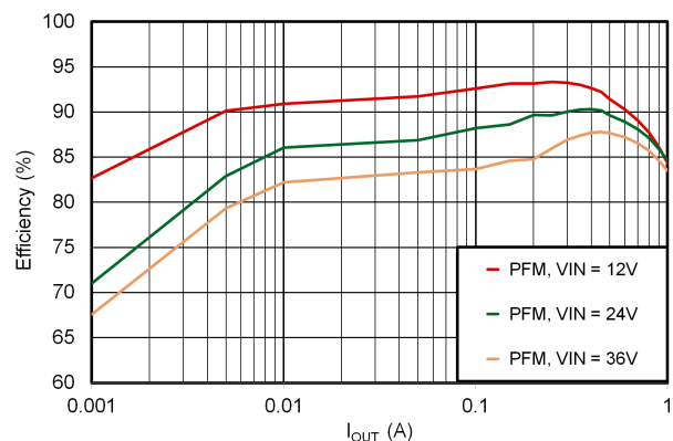
Efficiency Versus Output Current V_{OUT} = 5V, 400kHz
