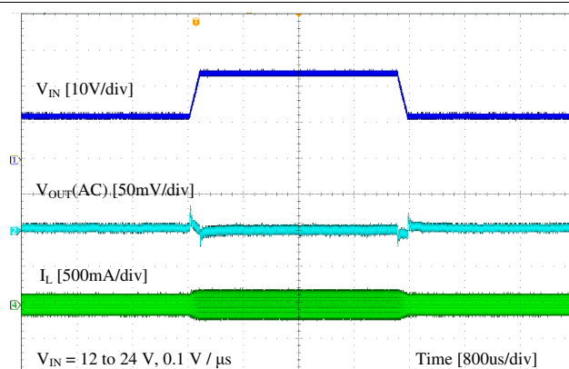
Figure 9-7. Line Transient
