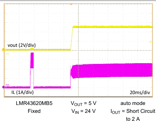
Figure 9-13. Short-Circuit Recovery
