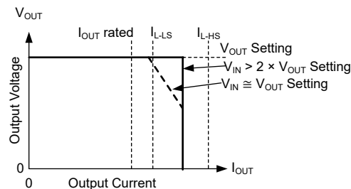
Figure 8-14. Output Voltage Versus Output Current
