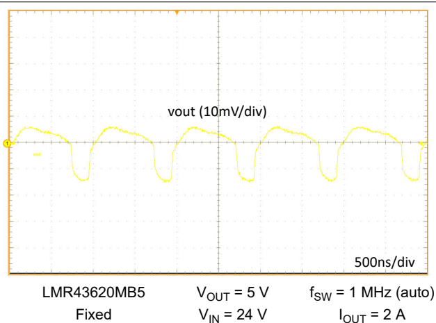
Figure 9-14. Output Voltage Ripple
