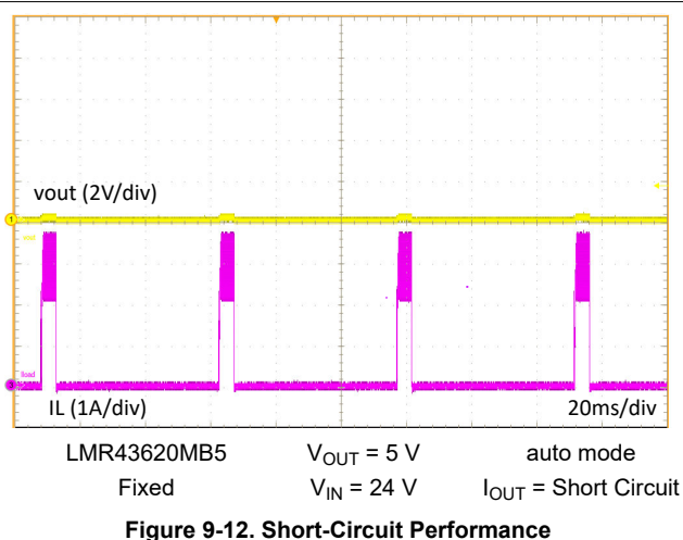
Figure 9-12. Short-Circuit Performance
