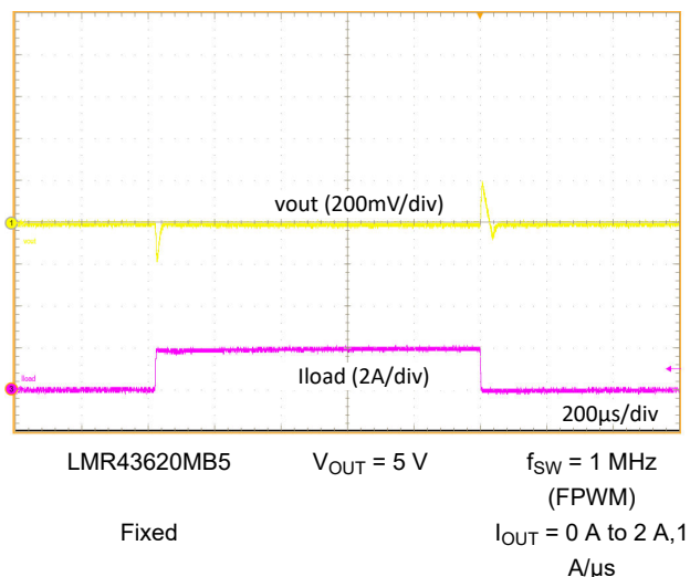
Figure 9-10. Load Transient
