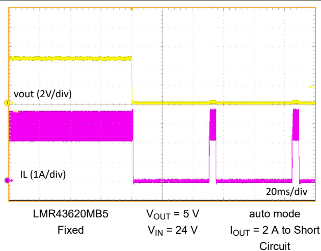
Figure 9-11. Short-Circuit Protection
