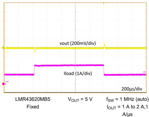
Figure 9-9. Load Transient
