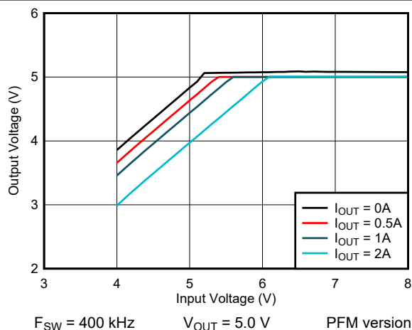
Figure 7-3. 5-V Dropout
