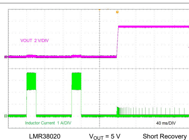
Figure 9-8. Short-Circuit Recovery
