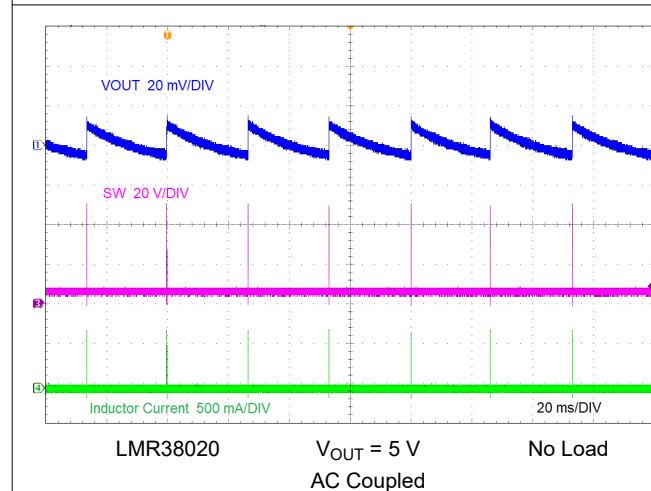
Figure 9-5. PFM Switching
