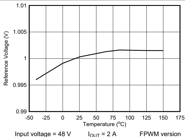
Figure 7-4. Reference Voltage vs Temperature
