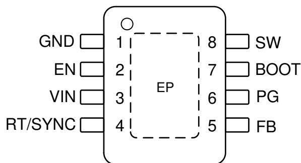
Figure 6-1. DDA Package, 8-Pin HSOIC (Top View)
