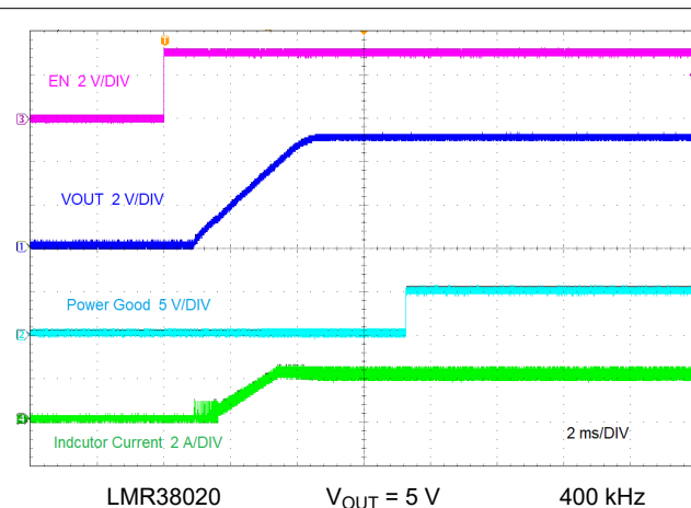
Figure 9-4. Start-Up by EN
