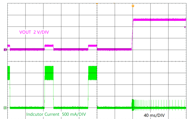
LMR38010-Q1 V_{OUT} = 5\text{ V} Short Recovery
