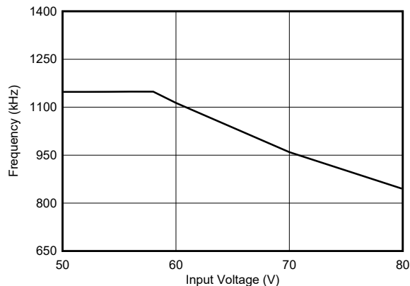
Figure 7-8. Typical Frequency Foldback at T_{ON\_MIN}
