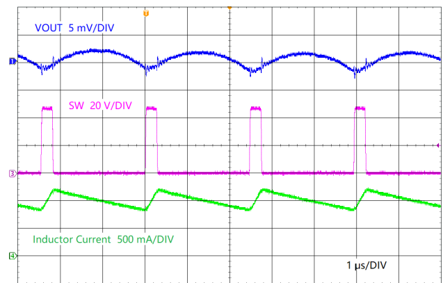
LMR38010-Q1 V_{OUT} = 5\text{ V} 400 kHz AC Coupled
