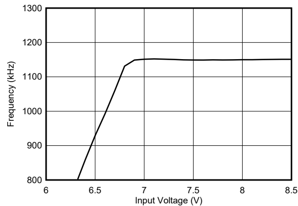
Figure 7-9. Typical Frequency Foldback at T_{OFF\_MIN}
