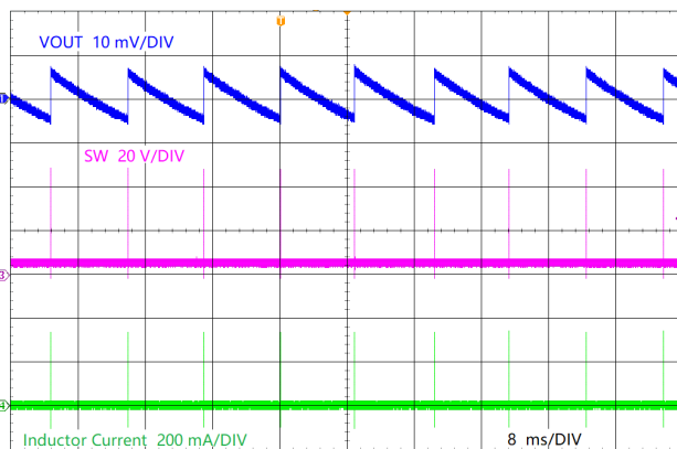
LMR38010-Q1 V_{OUT} = 5\text{ V} No Load AC Coupled
