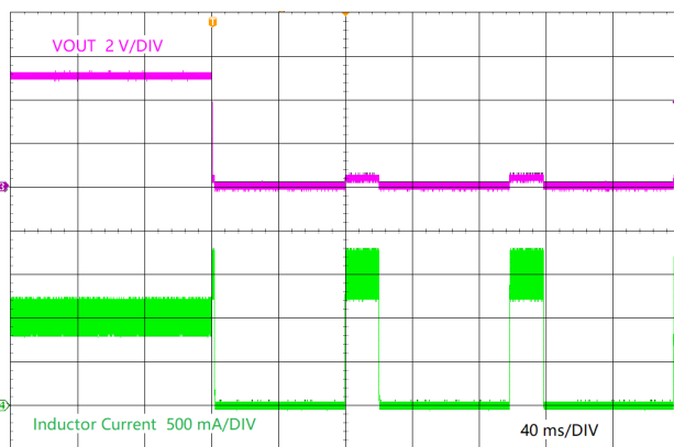
LMR38010-Q1 V_{OUT} = 5\text{ V} 1 A to Short
