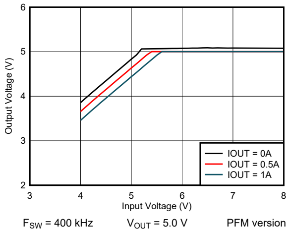
Figure 6-3. 5-V Dropout
