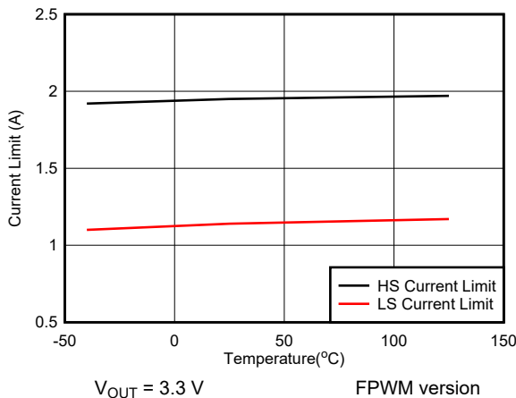
Figure 6-5. High-Side and Low-Side Current Limit vs Temperature
