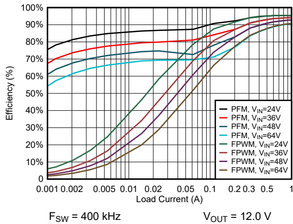
Figure 6-1. Efficiency vs Load Current
