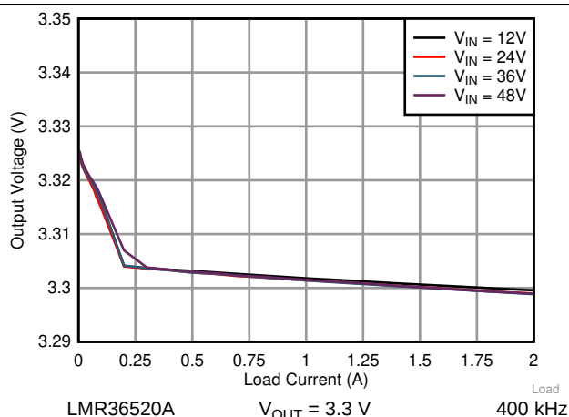
Figure 17. Load Regulation
