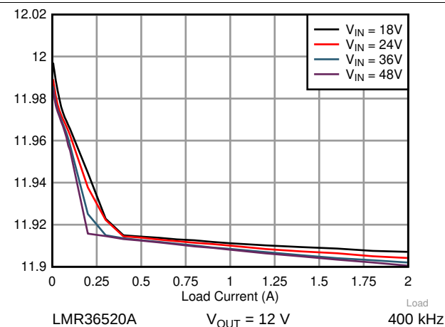
Figure 21. Load Regulation
