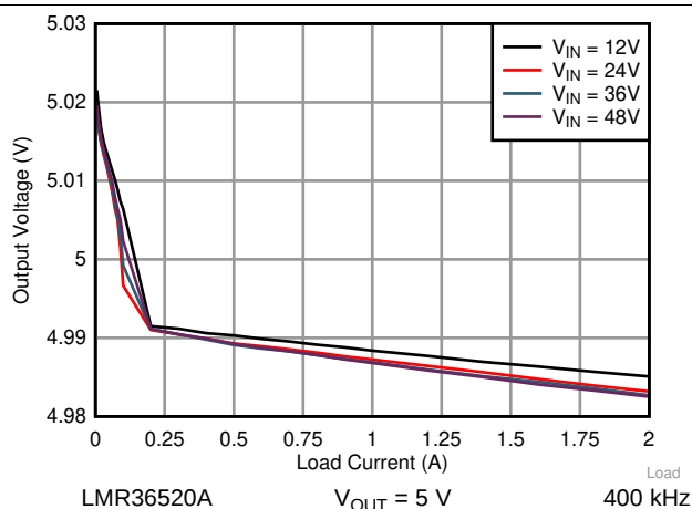
Figure 19. Load Regulation
