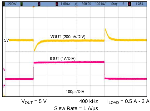
Figure 29. Load Transient
