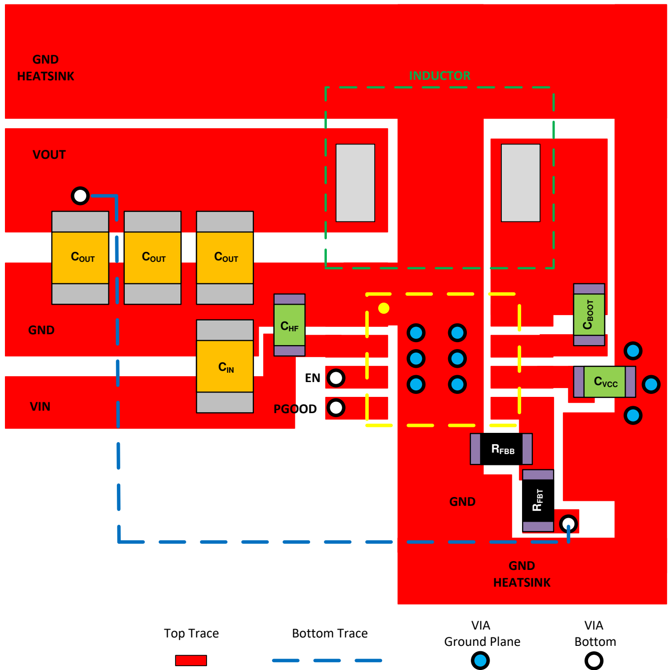
Figure 34. Example Layout
