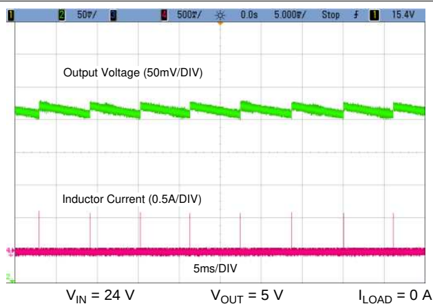
Figure 30. Output Ripple at No load
