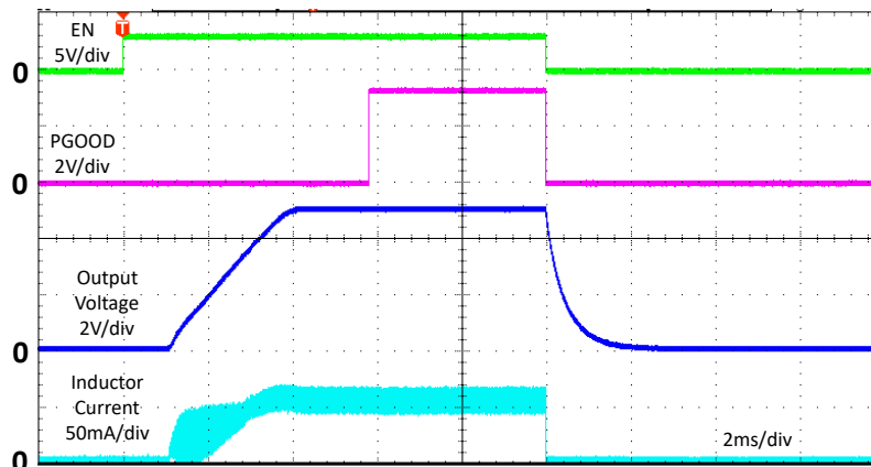
Figure 7-3. Enable Start-up V_{IN} = 24\text{ V} , V_{OUT} = 3.3\text{ V} , I_{OUT} = 50\text{ mA}
