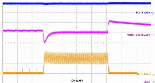
Figure 10-16. Load Transient
