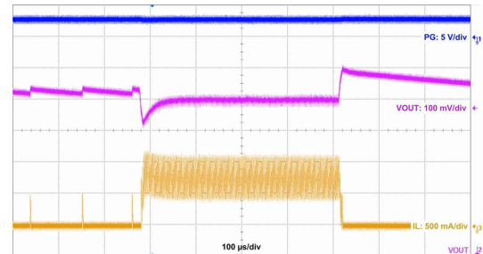
Figure 10-17. Load Transient
