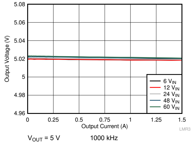
Figure 10-29. Load Regulation
