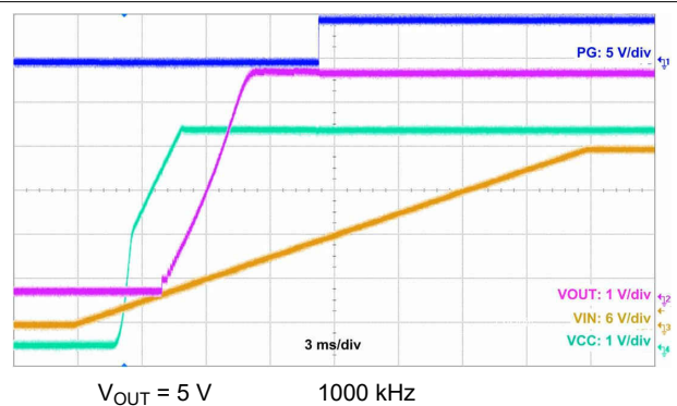
Figure 10-33. Start-Up Waveform
