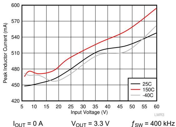
Figure 8-6. I_{PEAK-MIN}
