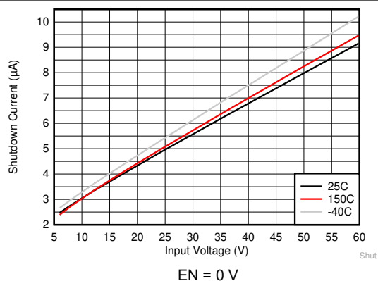
Figure 8-2. Shutdown Supply Current
