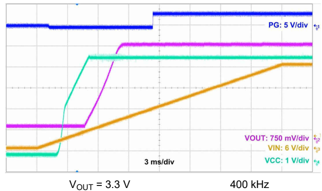
Figure 10-15. Start-Up Waveform
