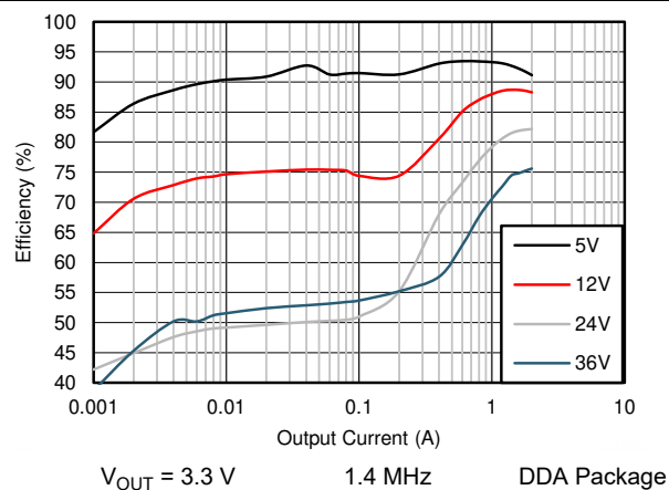
Figure 9-10. Efficiency
