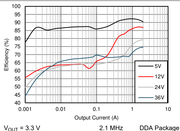
Figure 9-12. Efficiency
