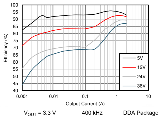
Figure 9-8. Efficiency
