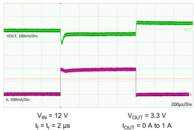
Figure 9-17. Load Transient
