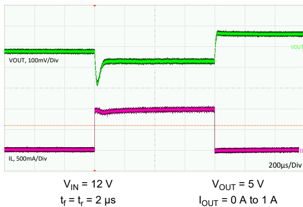
Figure 9-16. Load Transient
