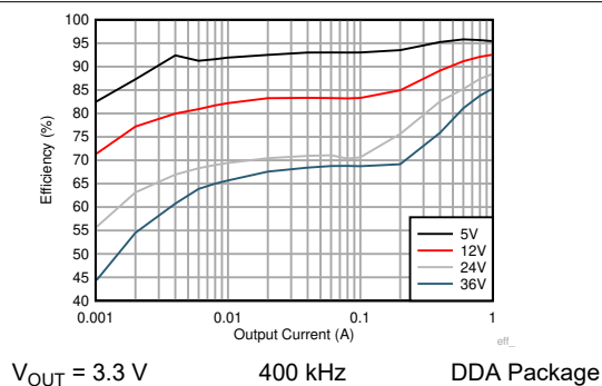
Figure 9-7. Efficiency
