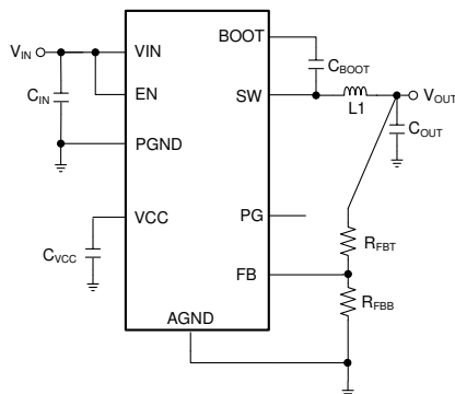
Simplified Schematic
