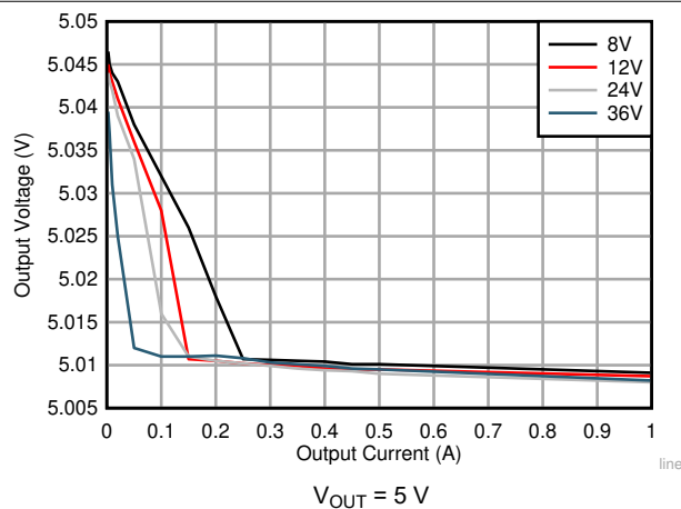
Figure 9-10. Line and Load Regulation
