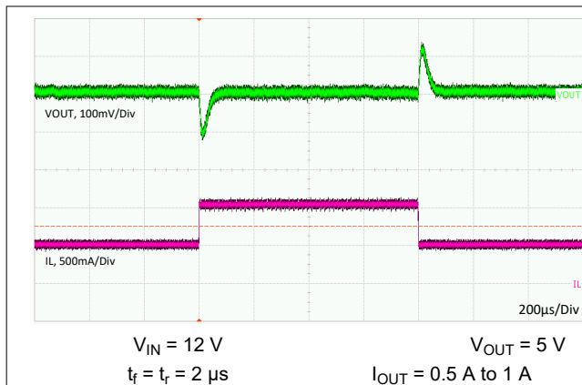
Figure 9-18. Load Transient
