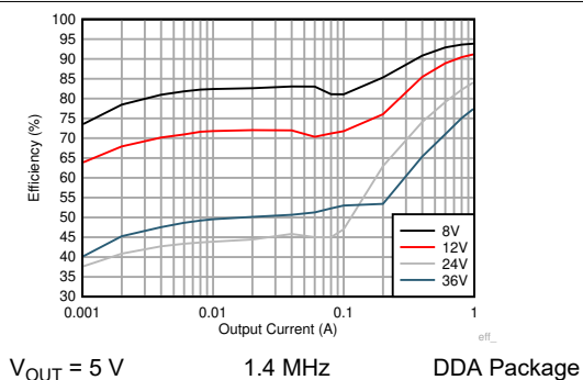
Figure 9-8. Efficiency
