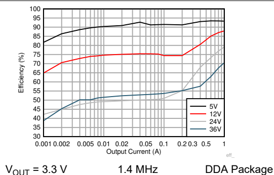
Figure 9-9. Efficiency
