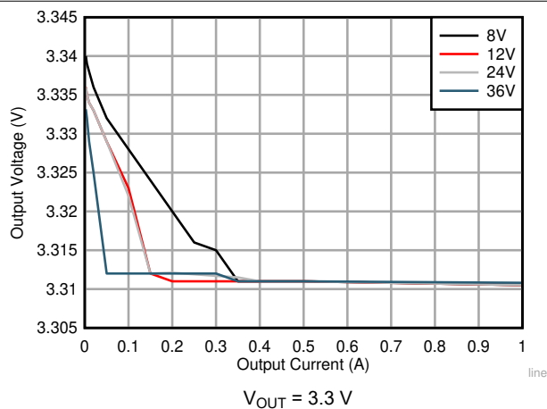
Figure 9-11. Line and Load Regulation
