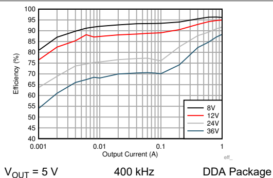
Figure 9-6. Efficiency
