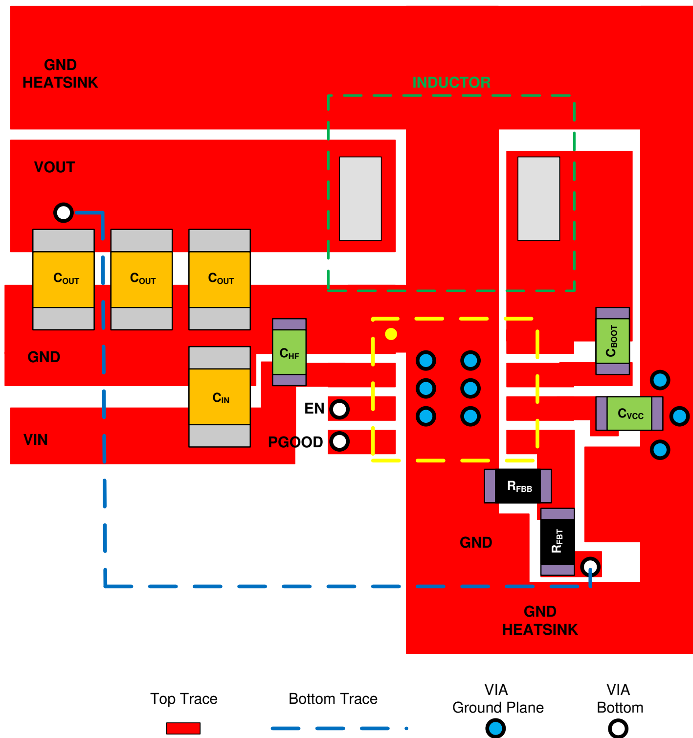
Figure 11-2. Example Layout for HSOIC (DDA) Package
