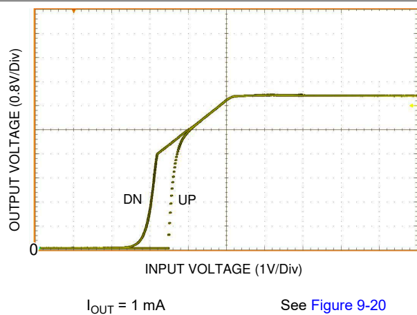
Figure 7-5. UVLO Thresholds
