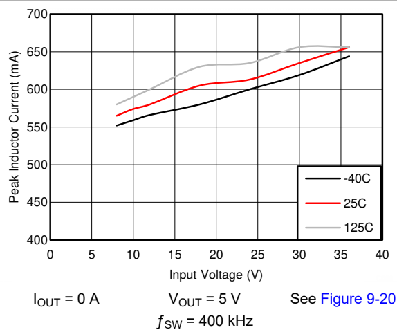
Figure 7-6. I_{PEAK-MIN}
