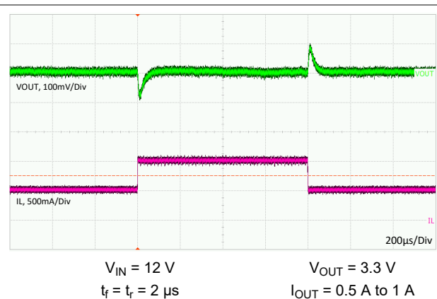
Figure 9-19. Load Transient
