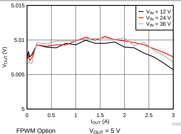
Figure 6. Load Regulation
