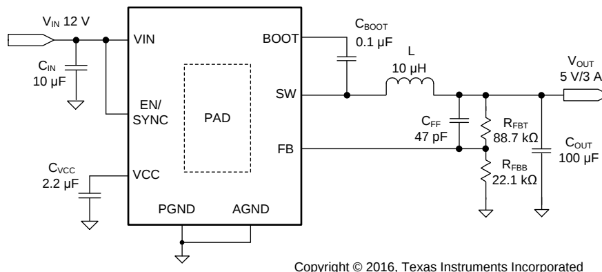
Figure 23. Application Circuit
