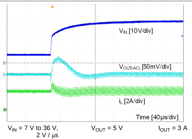
Figure 31. Line Transient
