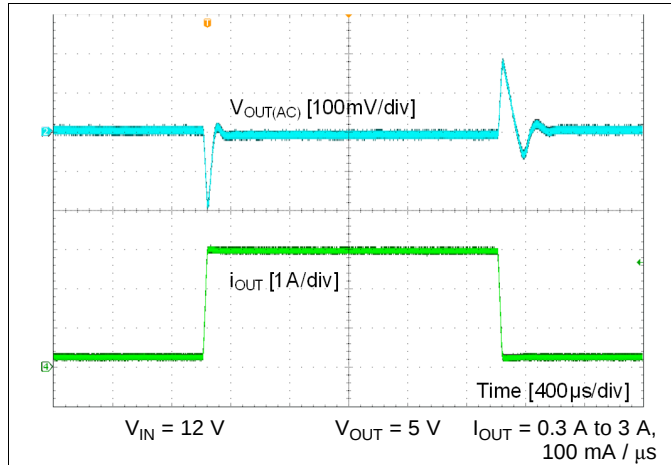
Figure 30. Load Transient
