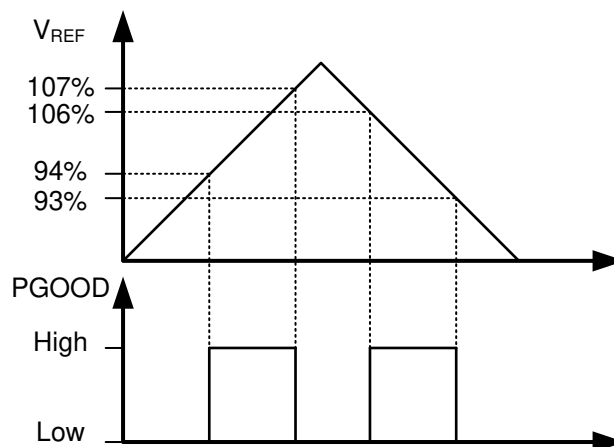
Figure 8-9. Power-Good Flag
