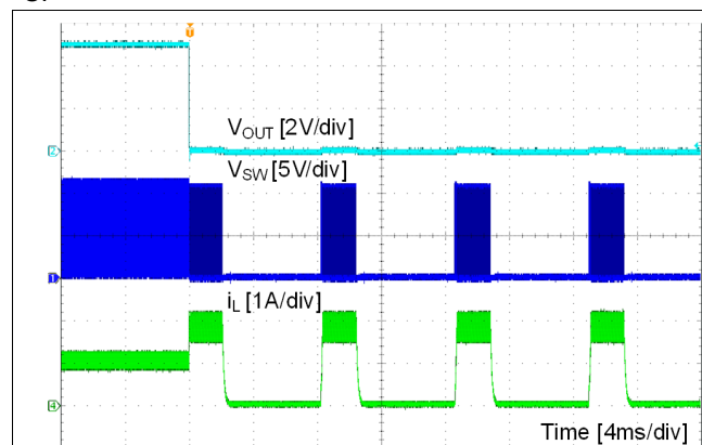
Figure 28. Short Protection
