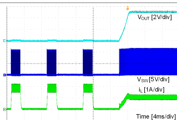
Figure 29. Short Recovery
