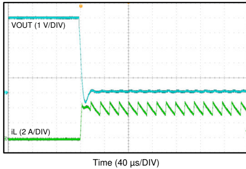
Figure 7-8. Output Short
