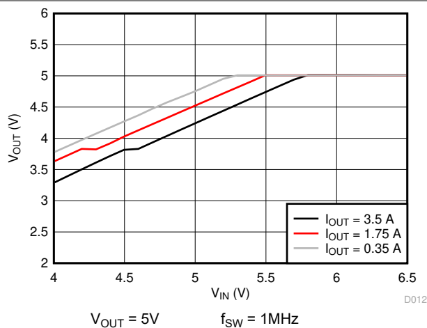
Figure 5-8. Dropout Curve
