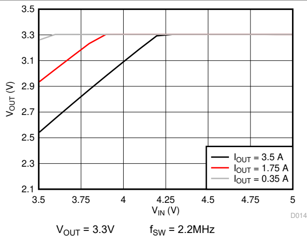
Figure 5-10. Dropout Curve
