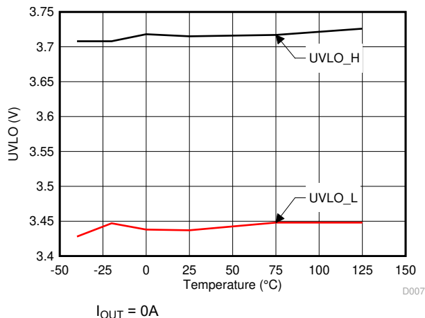
Figure 5-12. UVLO Threshold
